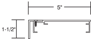
Standard Slide In Face
