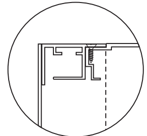
Aluminum Adhered to Retainer Monolithic Face
